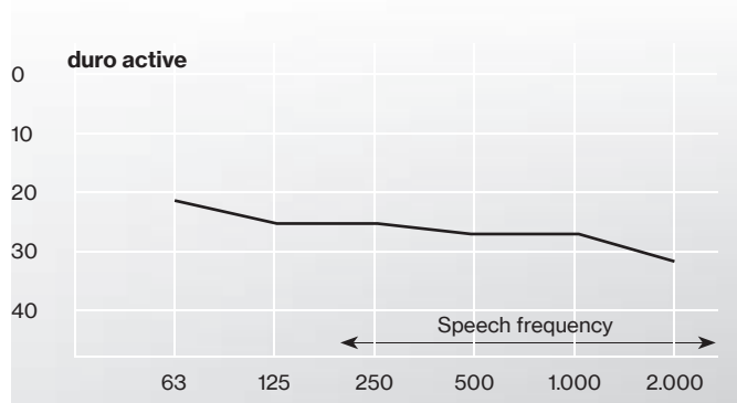
Frequency-dependent attenuation
