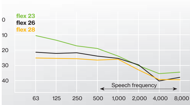
Frequency-dependent attenuation
