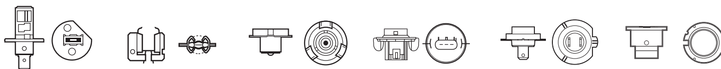
PI4,5s IEC 7004-46 X511 IEC 7004-99 P26s PX26d,4t IEC 7004-128-2 PX26d IEC 7004-5 P32d IEC 7004-111
