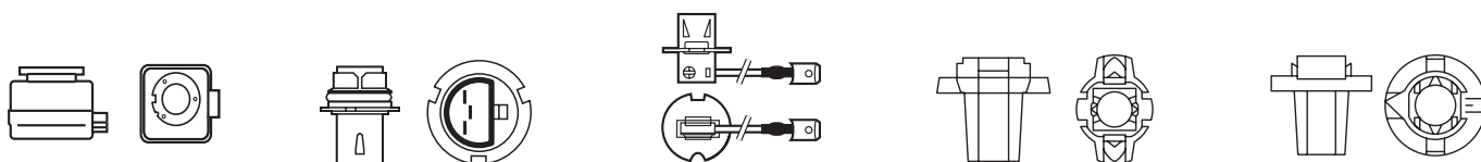
PK32d IEC 7004-111 P29t - PX29t IEC 7004-66 PK22s IEC 7004-47 BAX8,3S BAX8,5D
